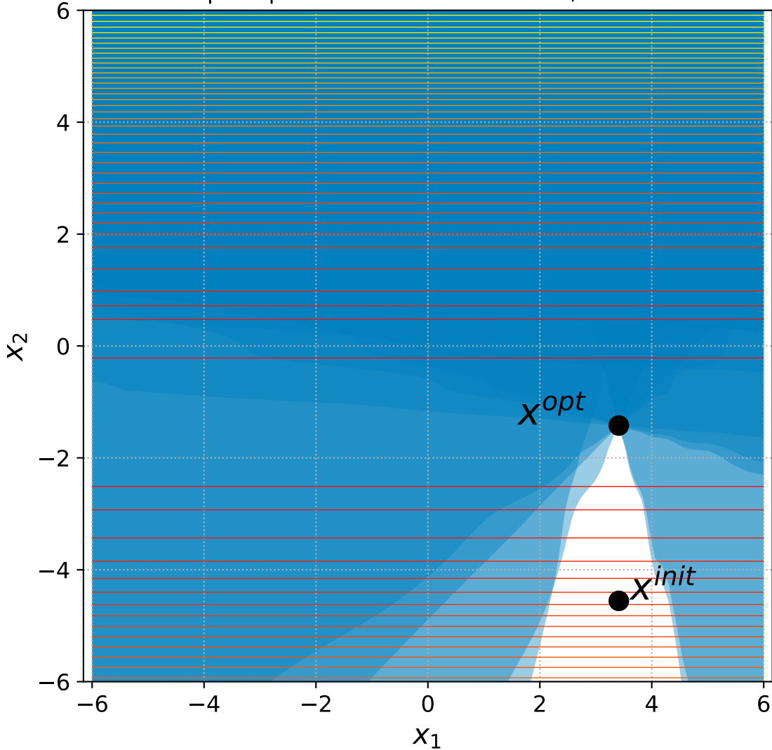
11 Sep. Ellipsoid with 6+n constraints, instance=5
