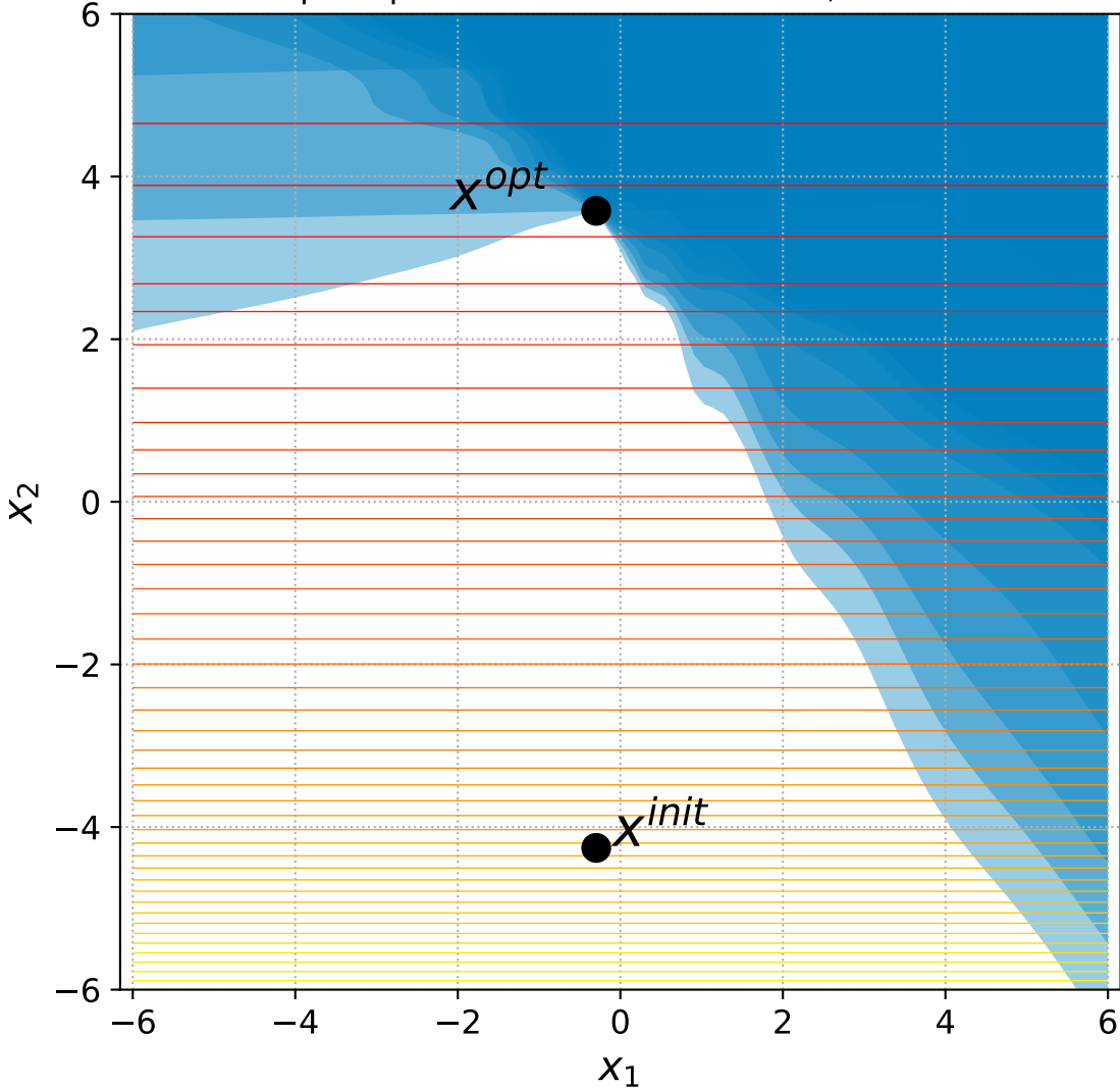
11 Sep. Ellipsoid with 6+n constraints, instance=4
