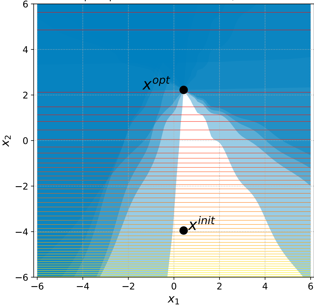
11 Sep. Ellipsoid with 6+n constraints, instance=3
