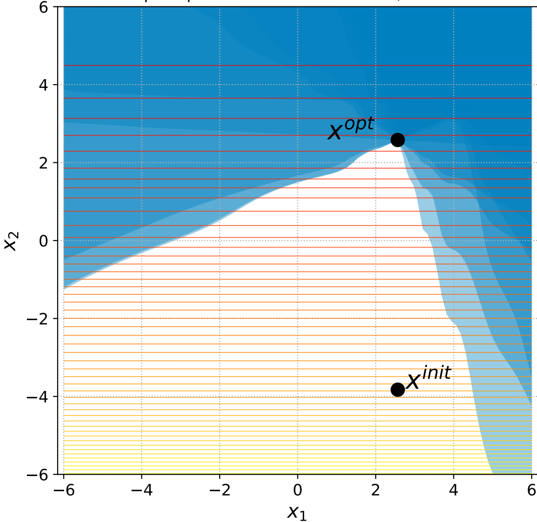
11 Sep. Ellipsoid with 6+n constraints, instance=2
