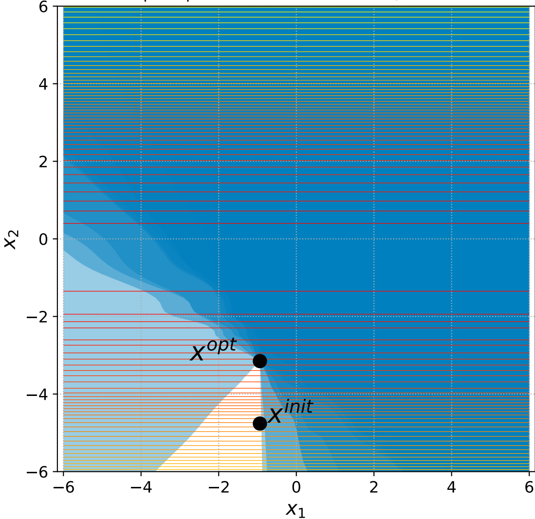
11 Sep. Ellipsoid with 6+n constraints, instance=1
