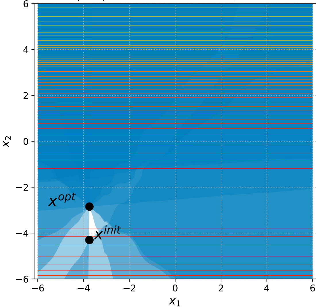
10 Sep. Ellipsoid with 6+n/2 constraints, instance=14
