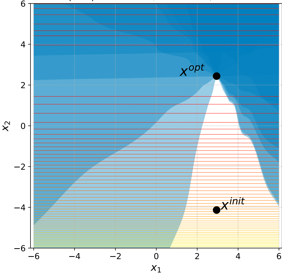
10 Sep. Ellipsoid with 6+n/2 constraints, instance=13
