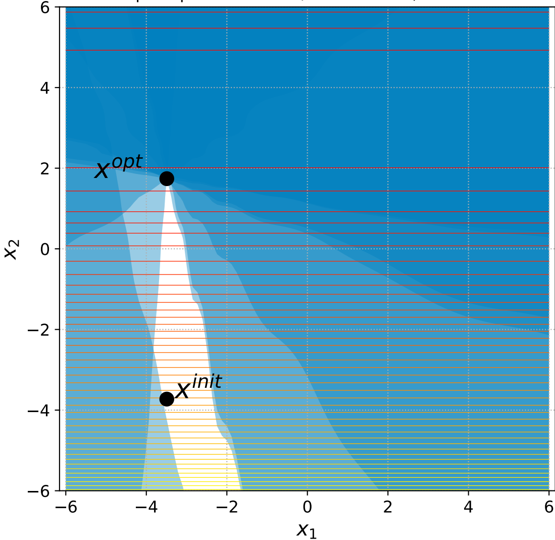
10 Sep. Ellipsoid with 6+n/2 constraints, instance=11
