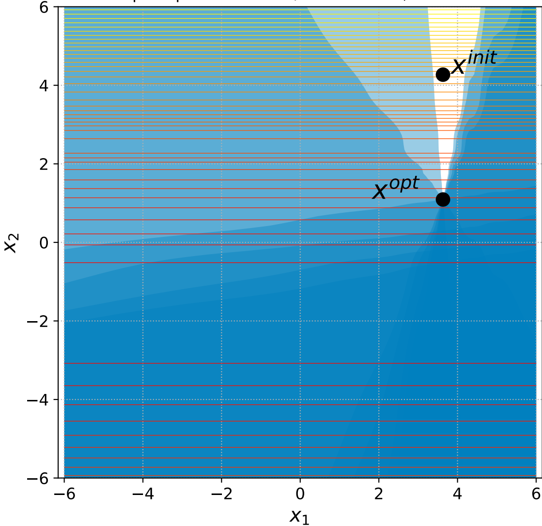
10 Sep. Ellipsoid with 6+n/2 constraints, instance=10
