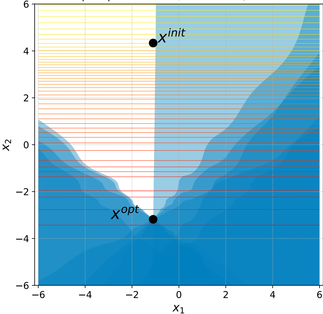
10 Sep. Ellipsoid with 6+n/2 constraints, instance=9
