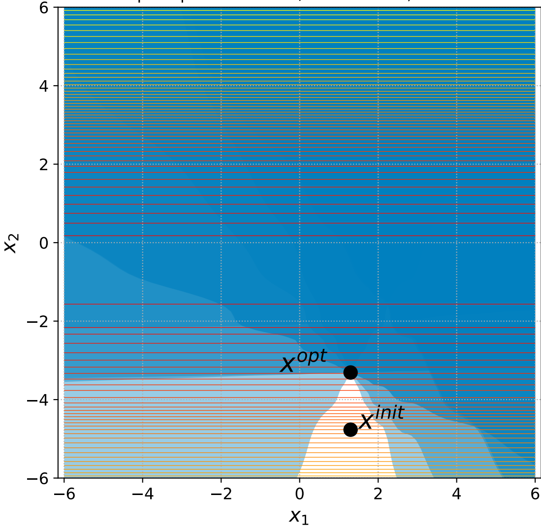
10 Sep. Ellipsoid with 6+n/2 constraints, instance=8
