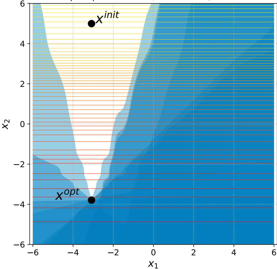
10 Sep. Ellipsoid with 6+n/2 constraints, instance=7
