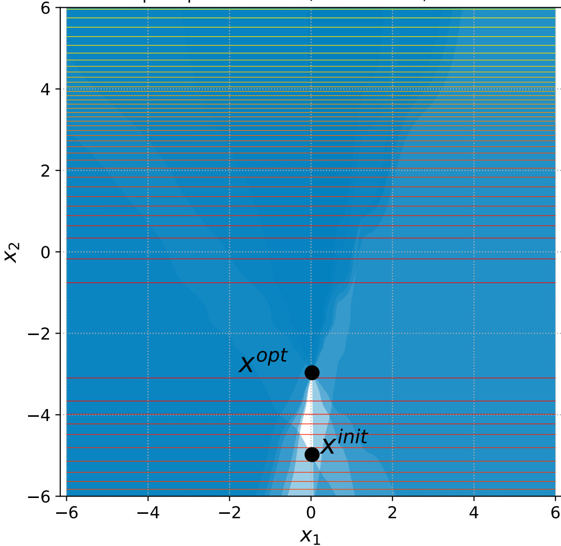
10 Sep. Ellipsoid with 6+n/2 constraints, instance=5
