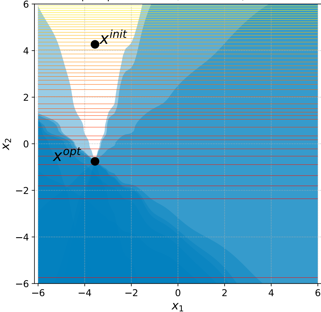
10 Sep. Ellipsoid with 6+n/2 constraints, instance=4
