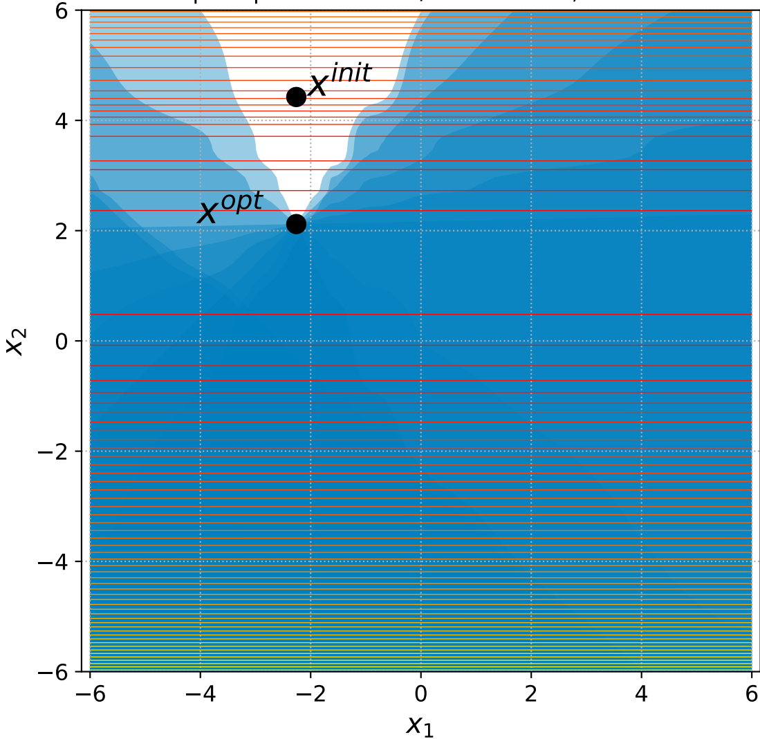
10 Sep. Ellipsoid with 6+n/2 constraints, instance=2
