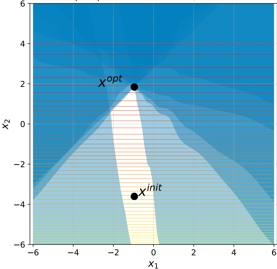
9 Sep. Ellipsoid with 6 constraints, instance=15
