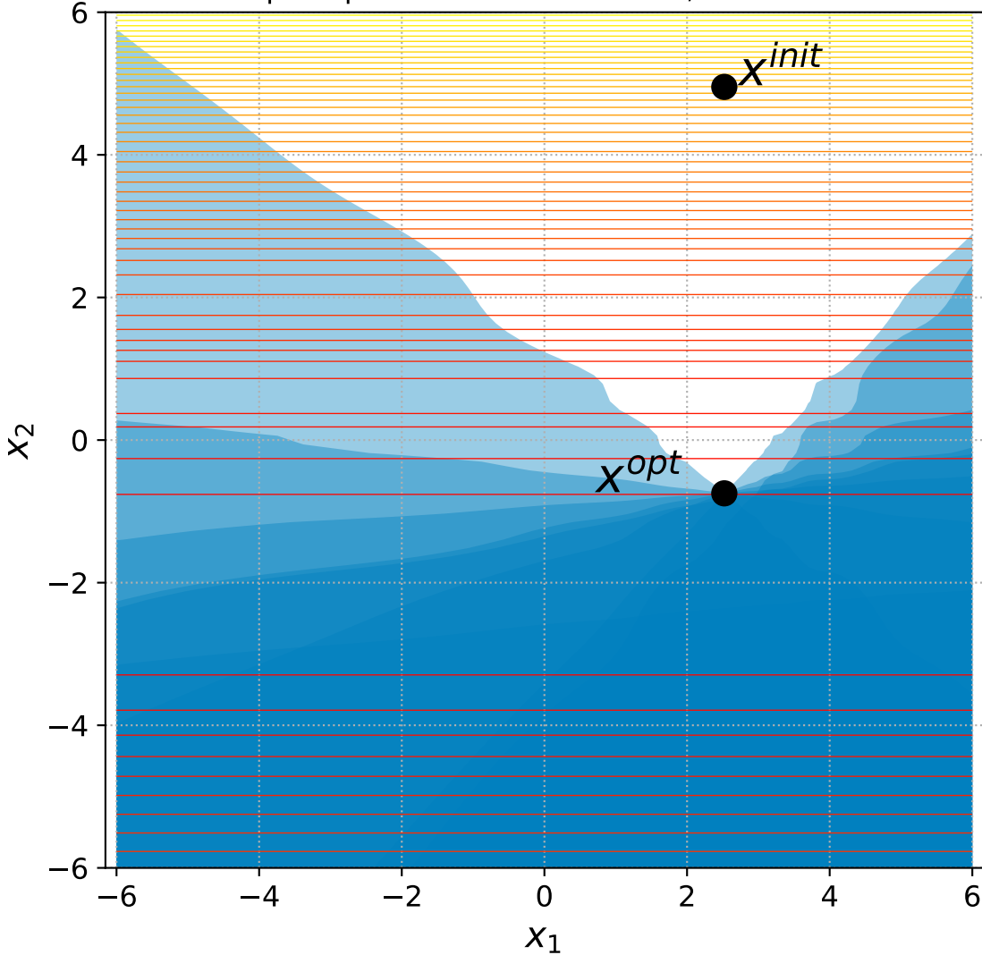
9 Sep. Ellipsoid with 6 constraints, instance=14
