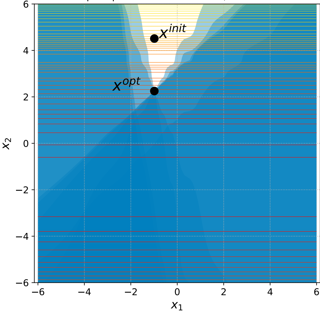
9 Sep. Ellipsoid with 6 constraints, instance=10
