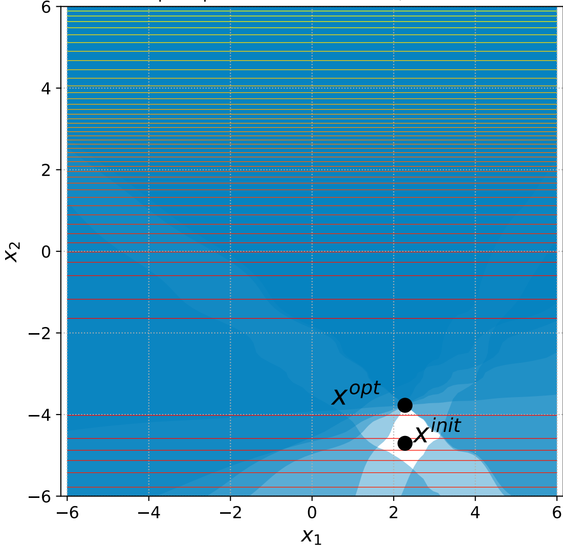
9 Sep. Ellipsoid with 6 constraints, instance=9
