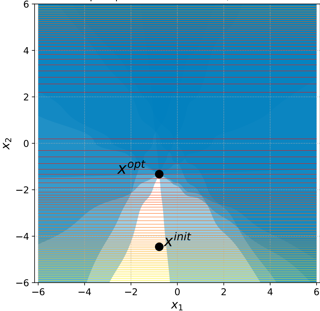
9 Sep. Ellipsoid with 6 constraints, instance=8
