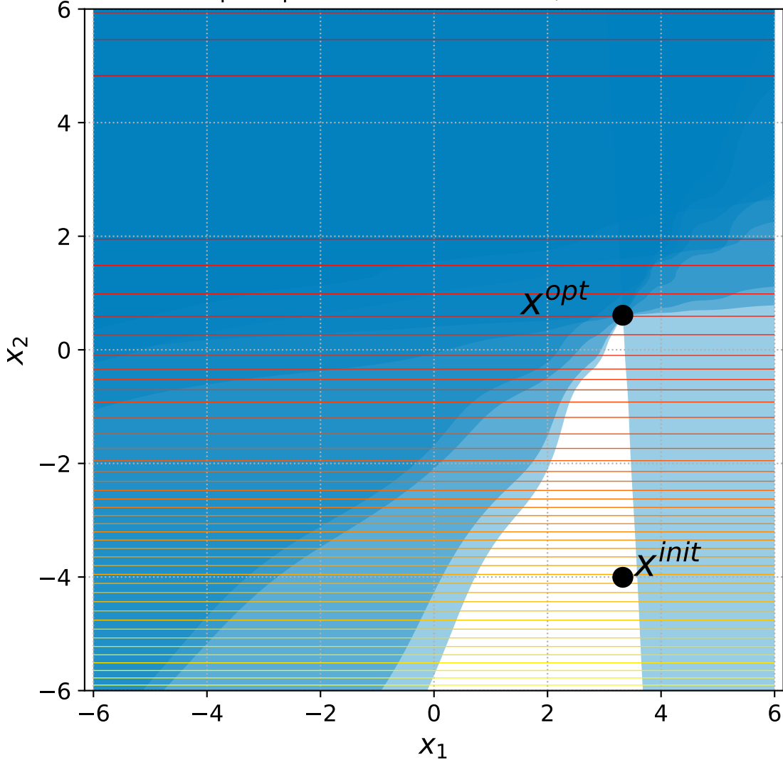
9 Sep. Ellipsoid with 6 constraints, instance=6
