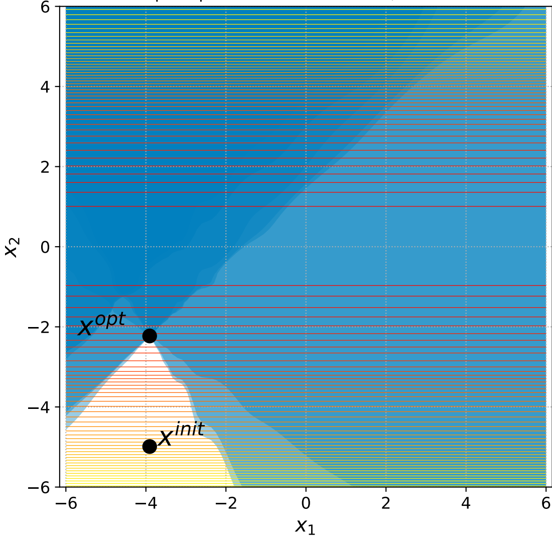
9 Sep. Ellipsoid with 6 constraints, instance=5
