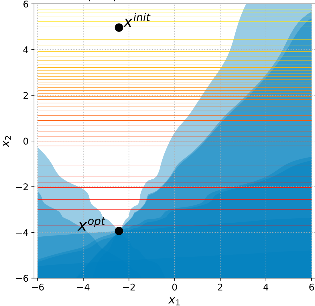
9 Sep. Ellipsoid with 6 constraints, instance=4
