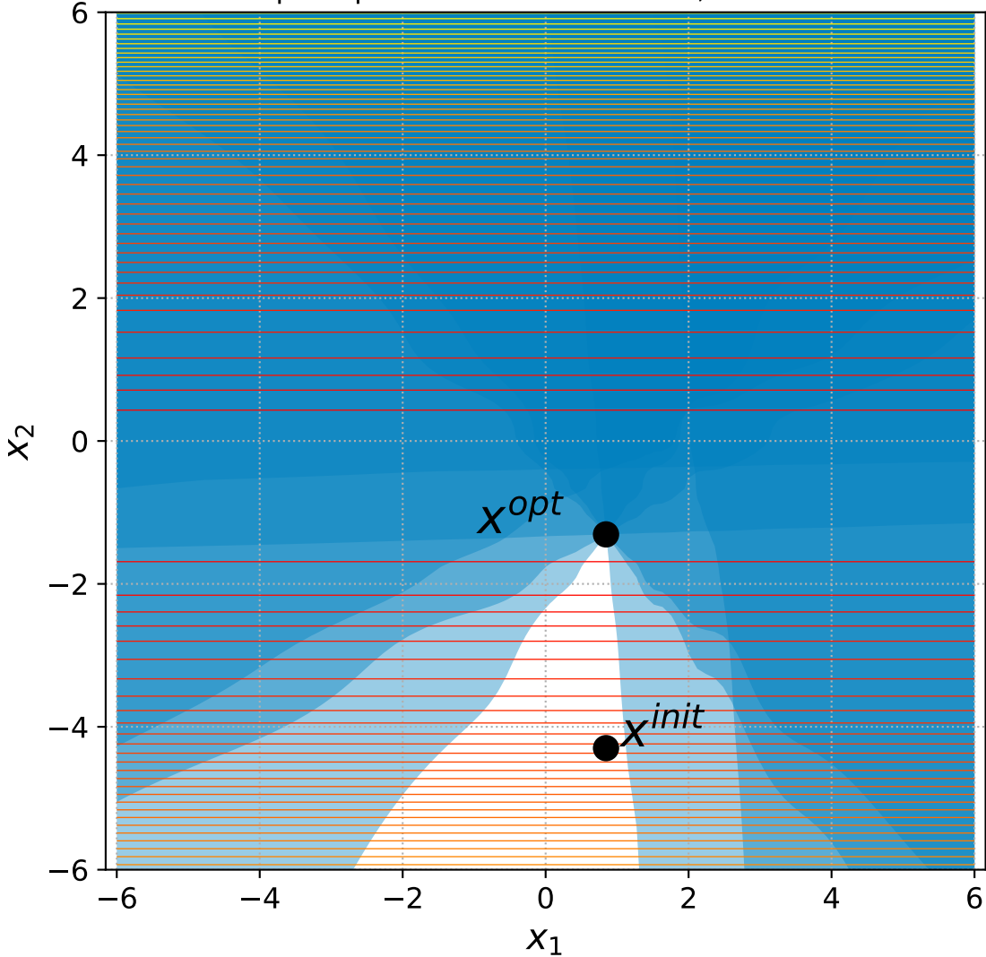
9 Sep. Ellipsoid with 6 constraints, instance=3
