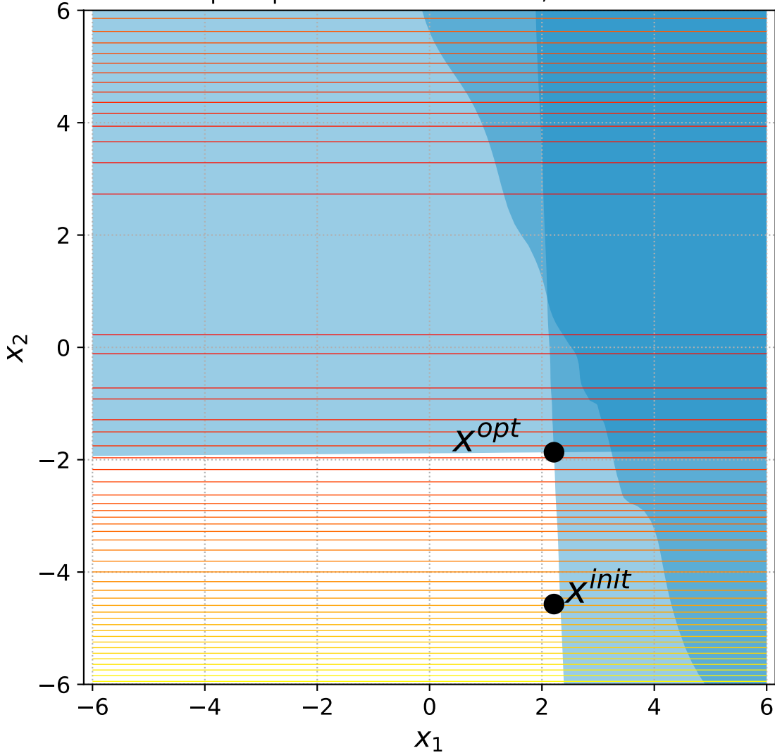
8 Sep. Ellipsoid with 2 constraints, instance=15
