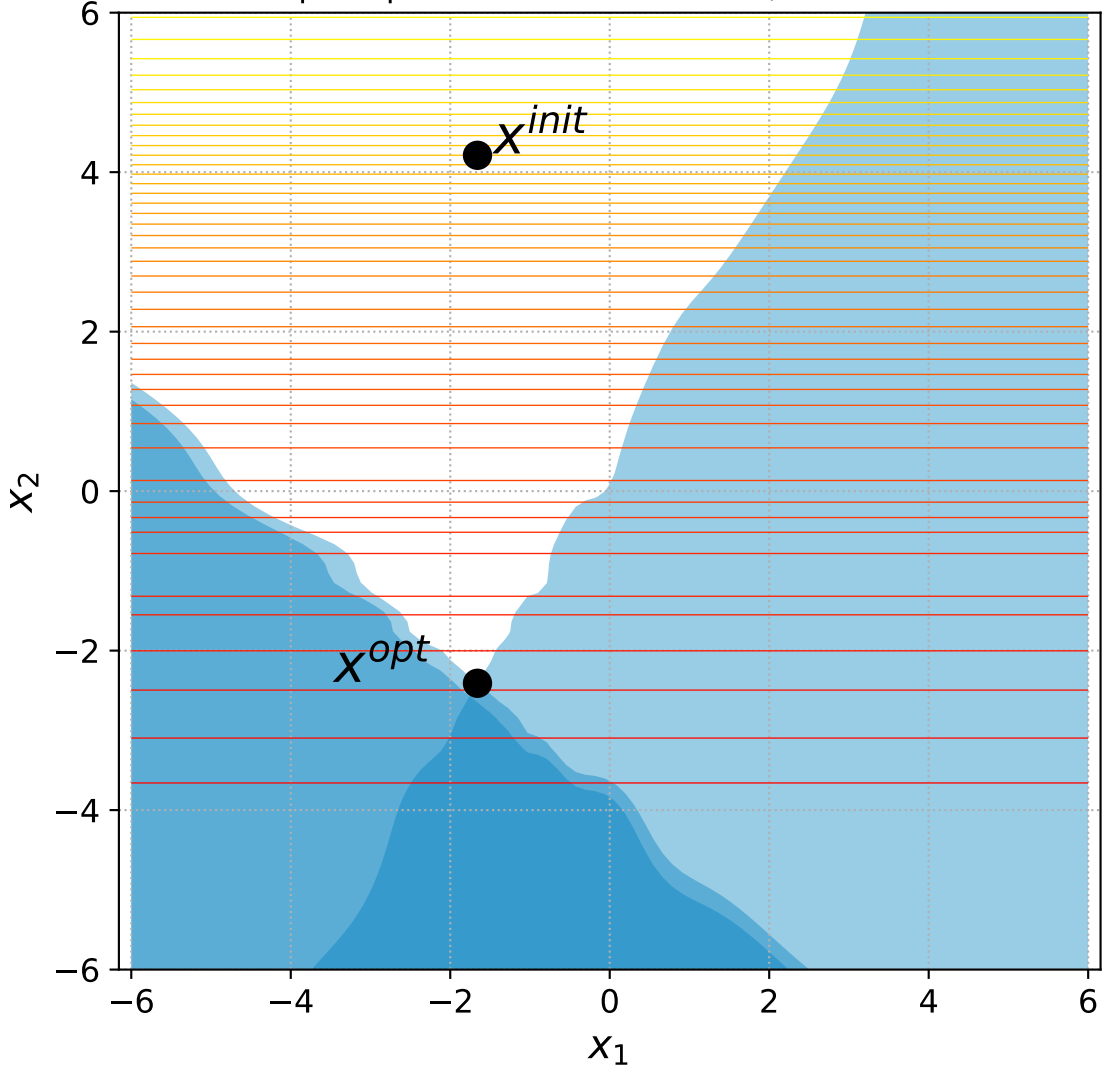
8 Sep. Ellipsoid with 2 constraints, instance=14
