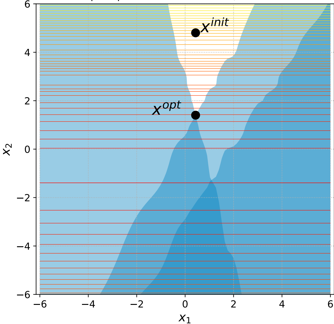
8 Sep. Ellipsoid with 2 constraints, instance=13
