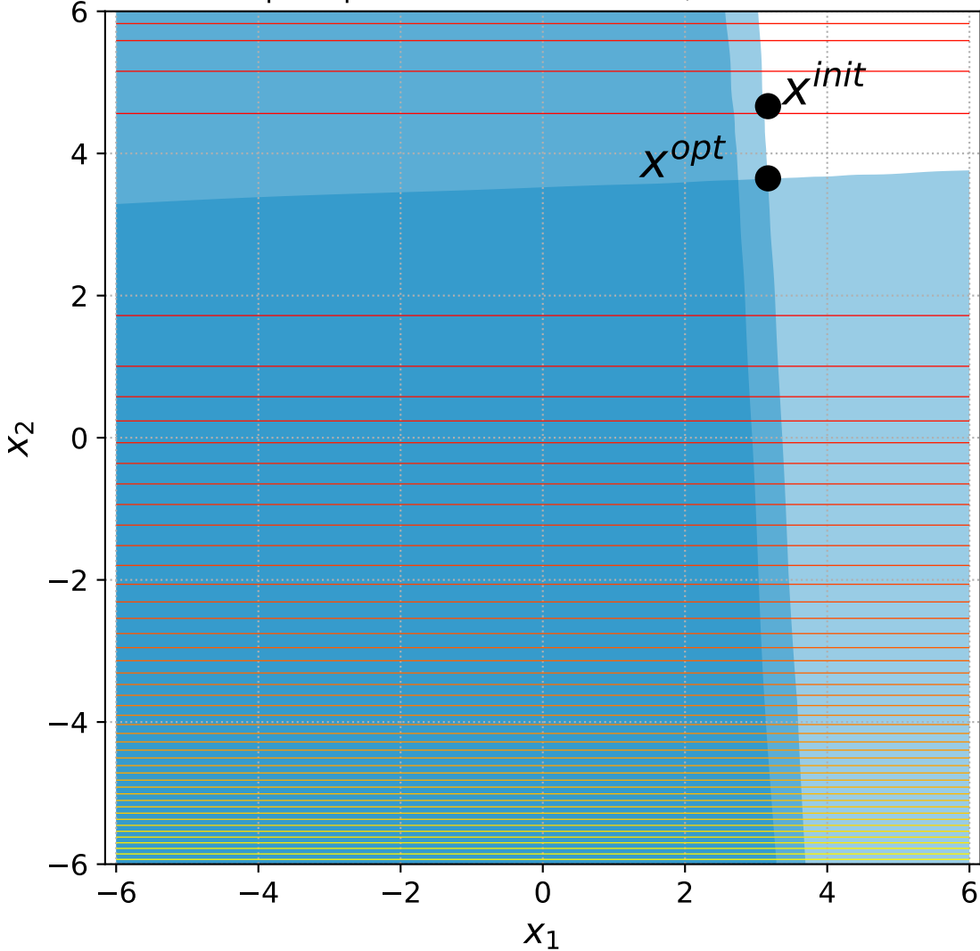
8 Sep. Ellipsoid with 2 constraints, instance=11
