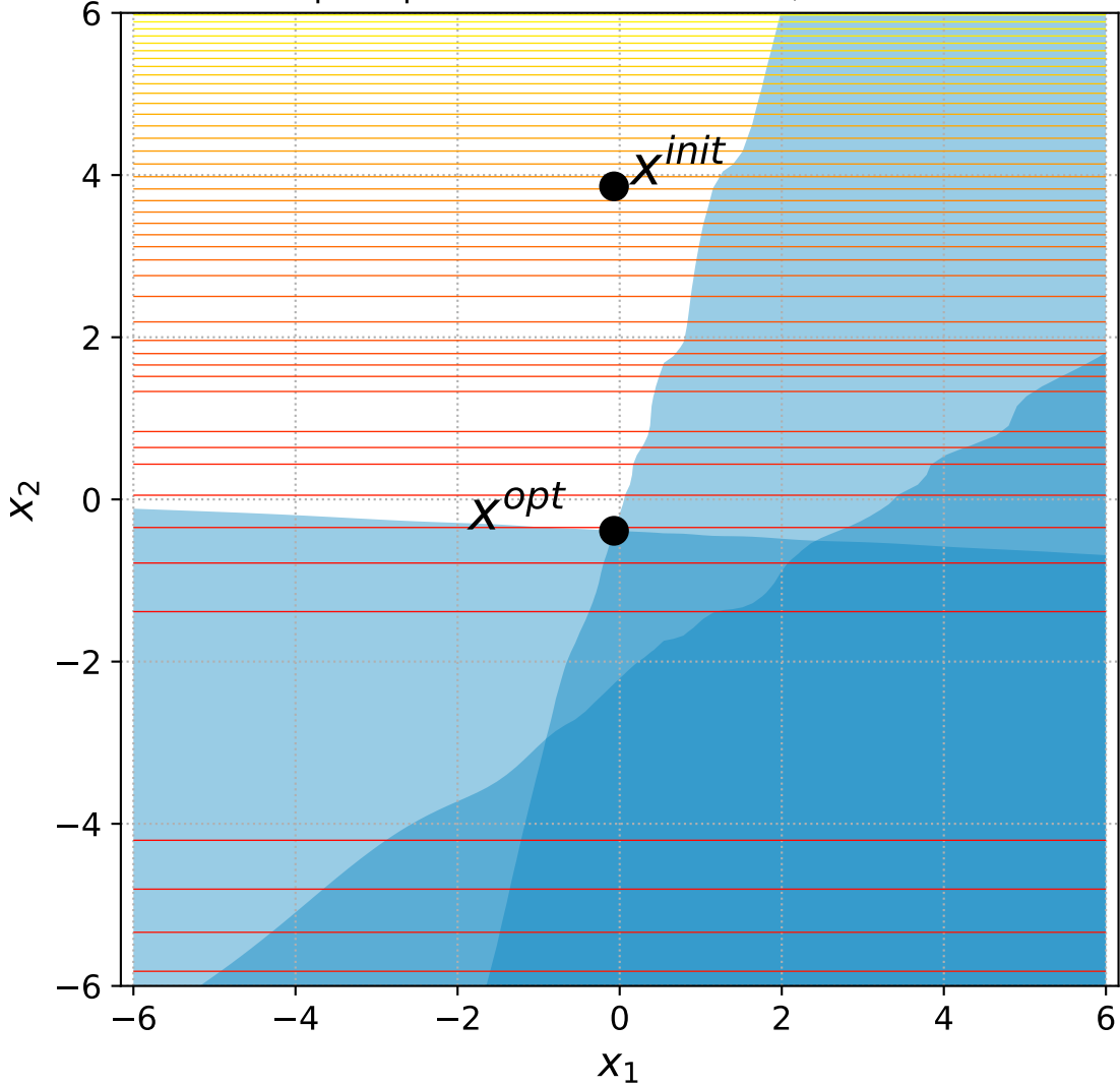
8 Sep. Ellipsoid with 2 constraints, instance=7
