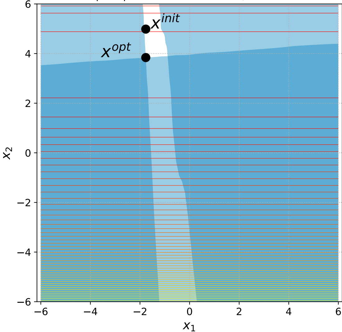
8 Sep. Ellipsoid with 2 constraints, instance=6
