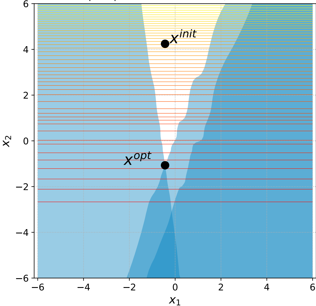
8 Sep. Ellipsoid with 2 constraints, instance=4
