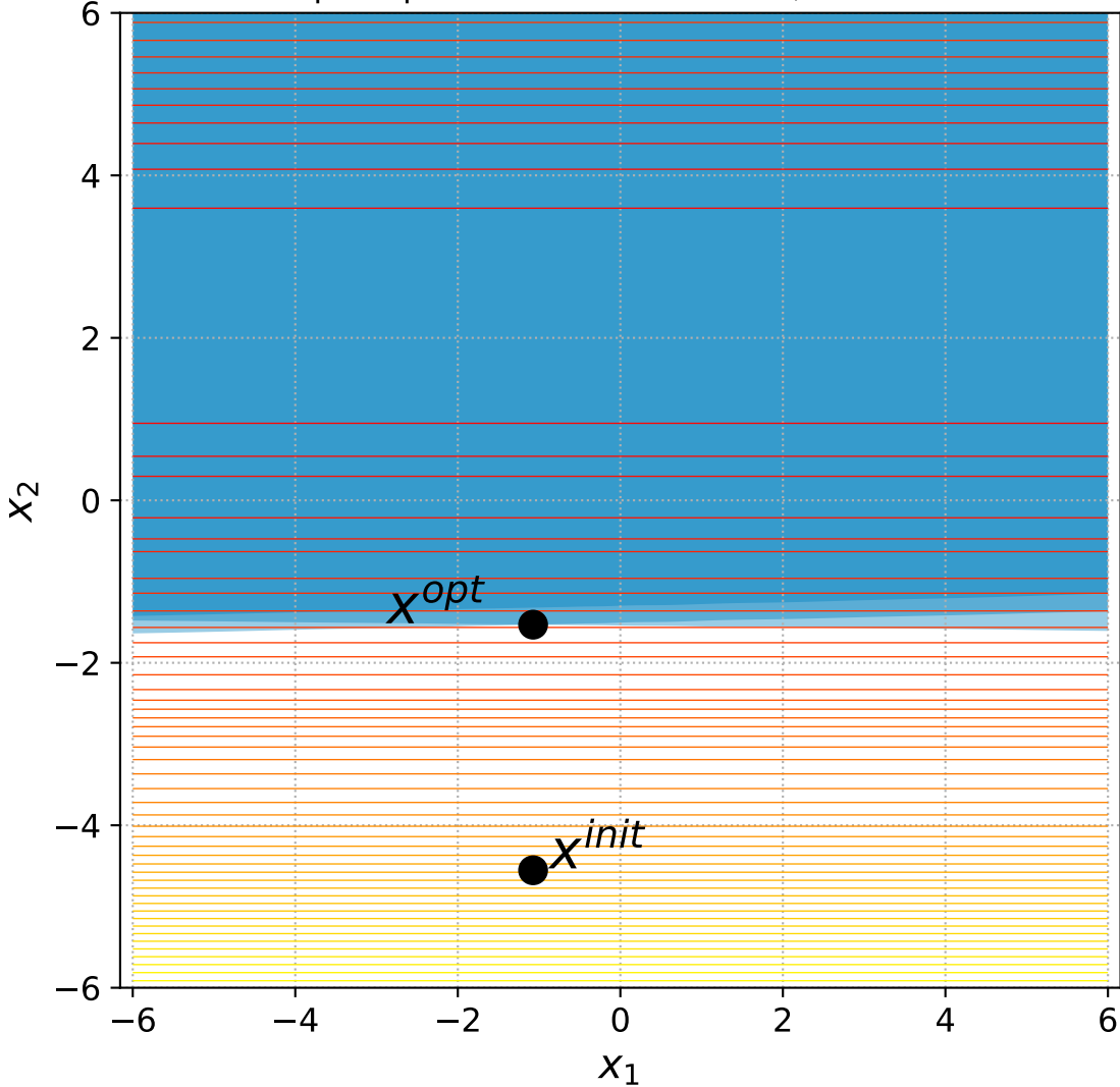
8 Sep. Ellipsoid with 2 constraints, instance=3
