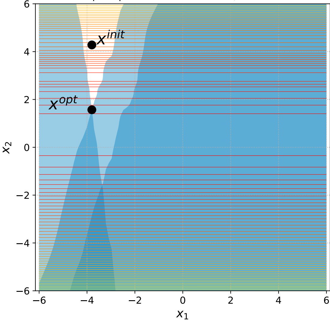
8 Sep. Ellipsoid with 2 constraints, instance=2
