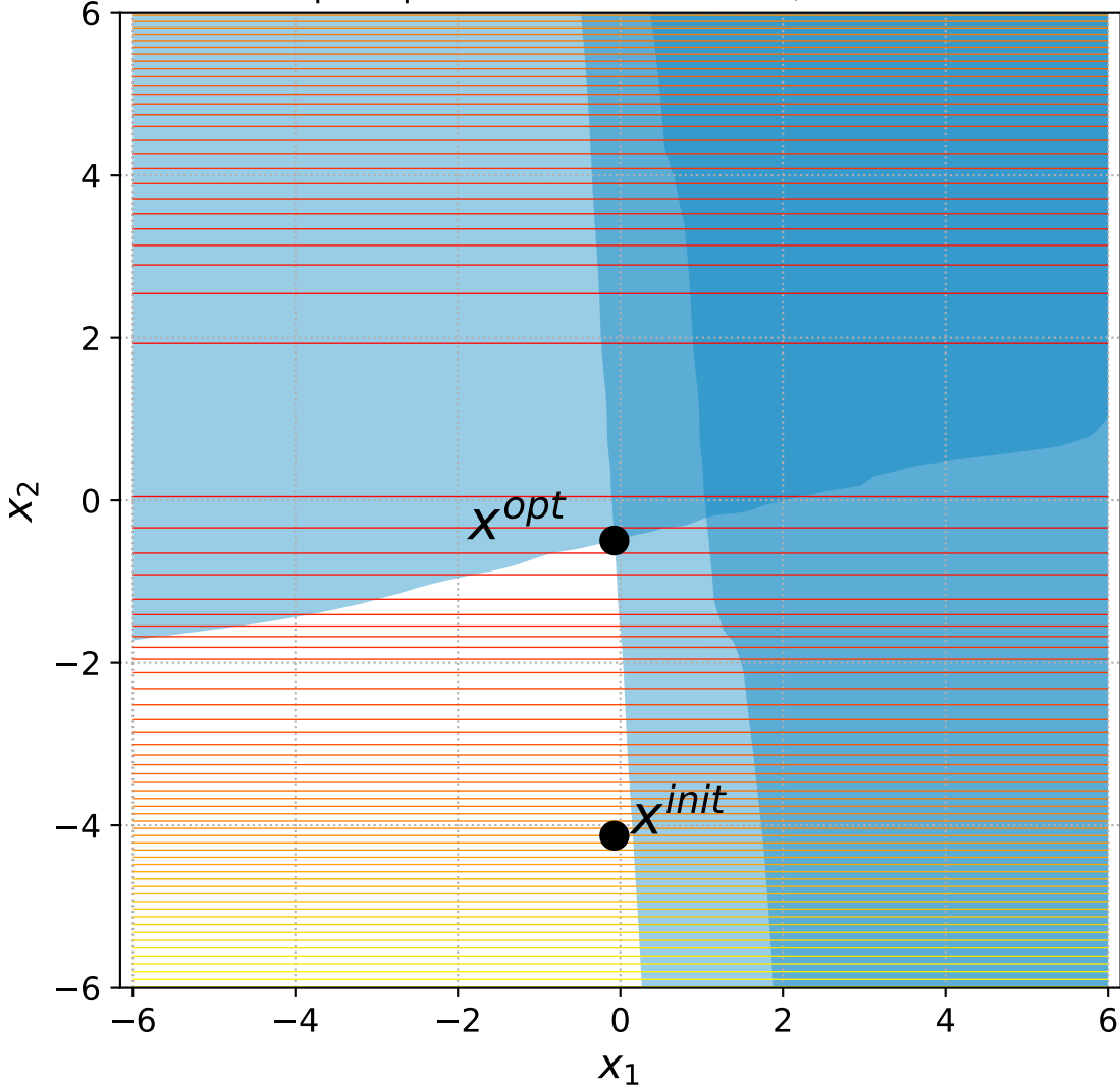
8 Sep. Ellipsoid with 2 constraints, instance=1
