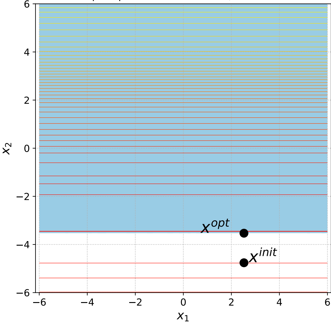
7 Sep. Ellipsoid with 1 constraint, instance=15
