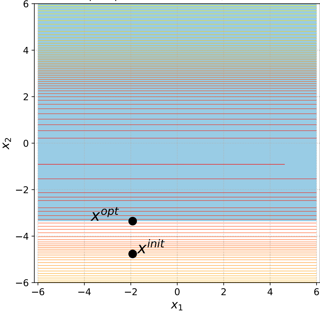
7 Sep. Ellipsoid with 1 constraint, instance=13
