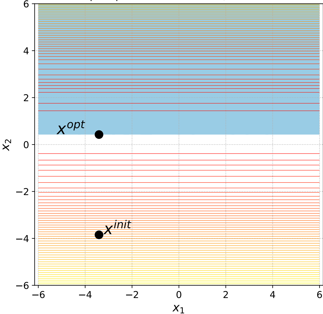
7 Sep. Ellipsoid with 1 constraint, instance=12
