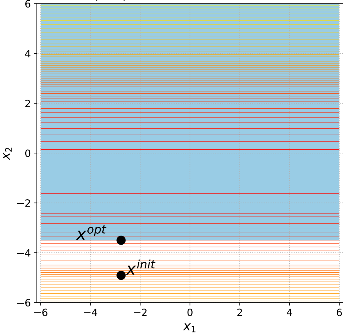
7 Sep. Ellipsoid with 1 constraint, instance=11
