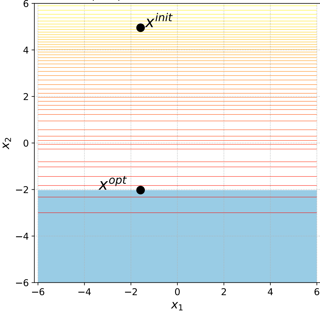
7 Sep. Ellipsoid with 1 constraint, instance=9
