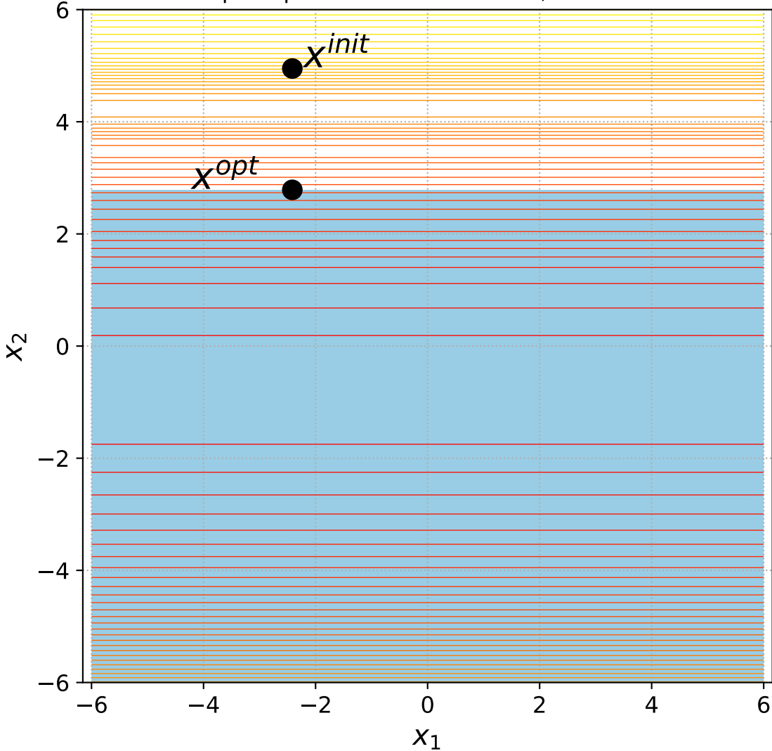
7 Sep. Ellipsoid with 1 constraint, instance=7
