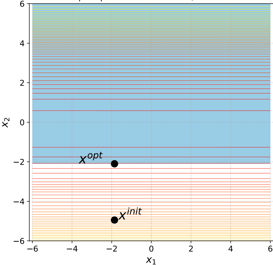
7 Sep. Ellipsoid with 1 constraint, instance=5
