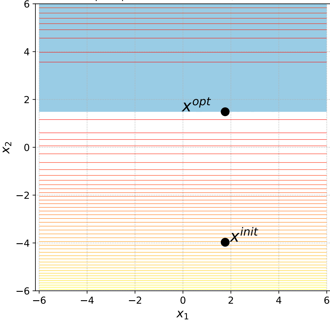
7 Sep. Ellipsoid with 1 constraint, instance=2
