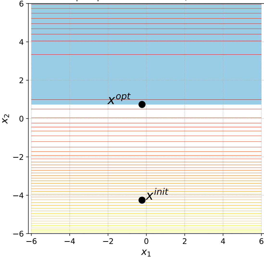
7 Sep. Ellipsoid with 1 constraint, instance=1
