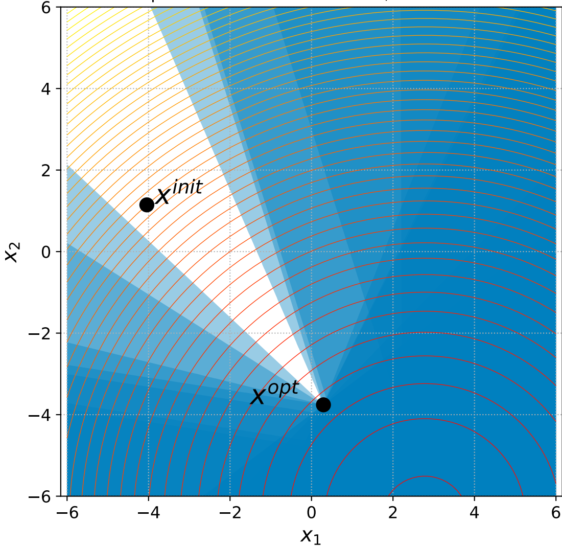
6 Sphere with 6+3n constraints, instance=15
