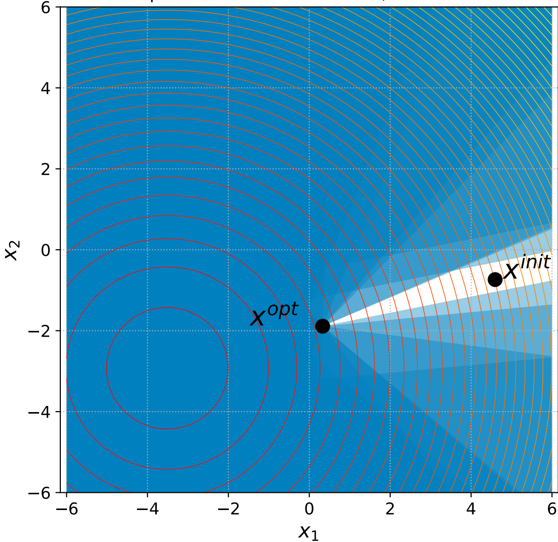
6 Sphere with 6+3n constraints, instance=14
