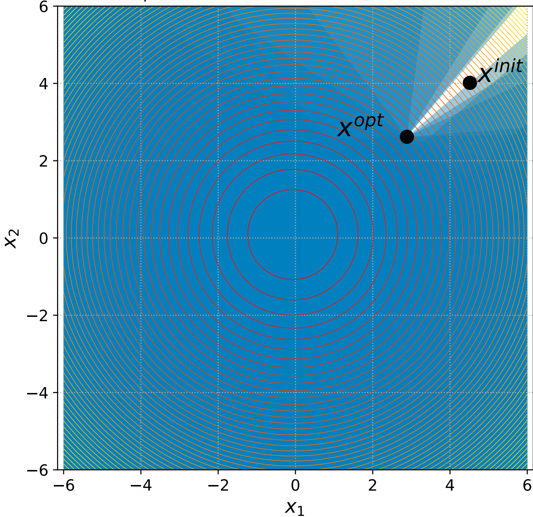
6 Sphere with 6+3n constraints, instance=12
