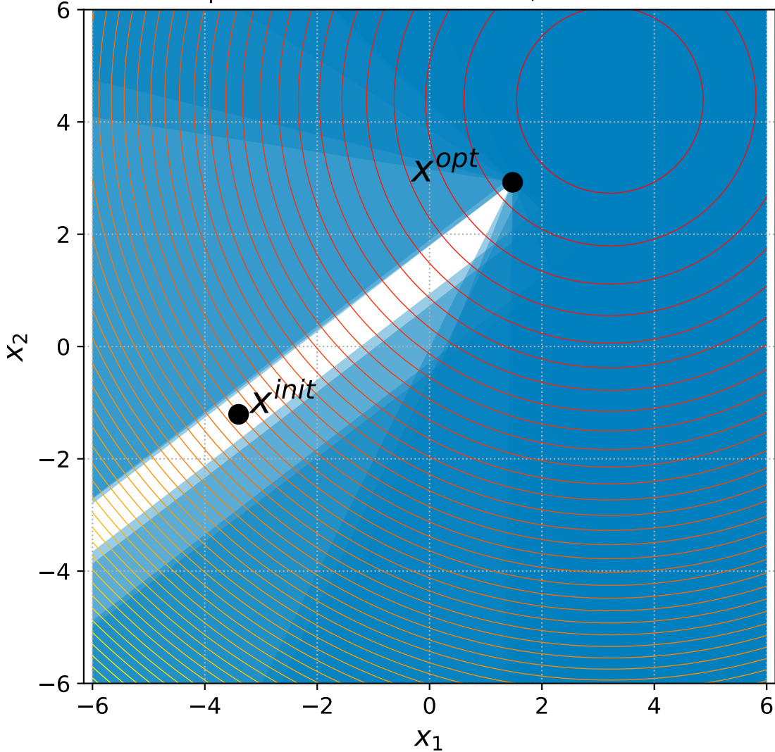
6 Sphere with 6+3n constraints, instance=10
