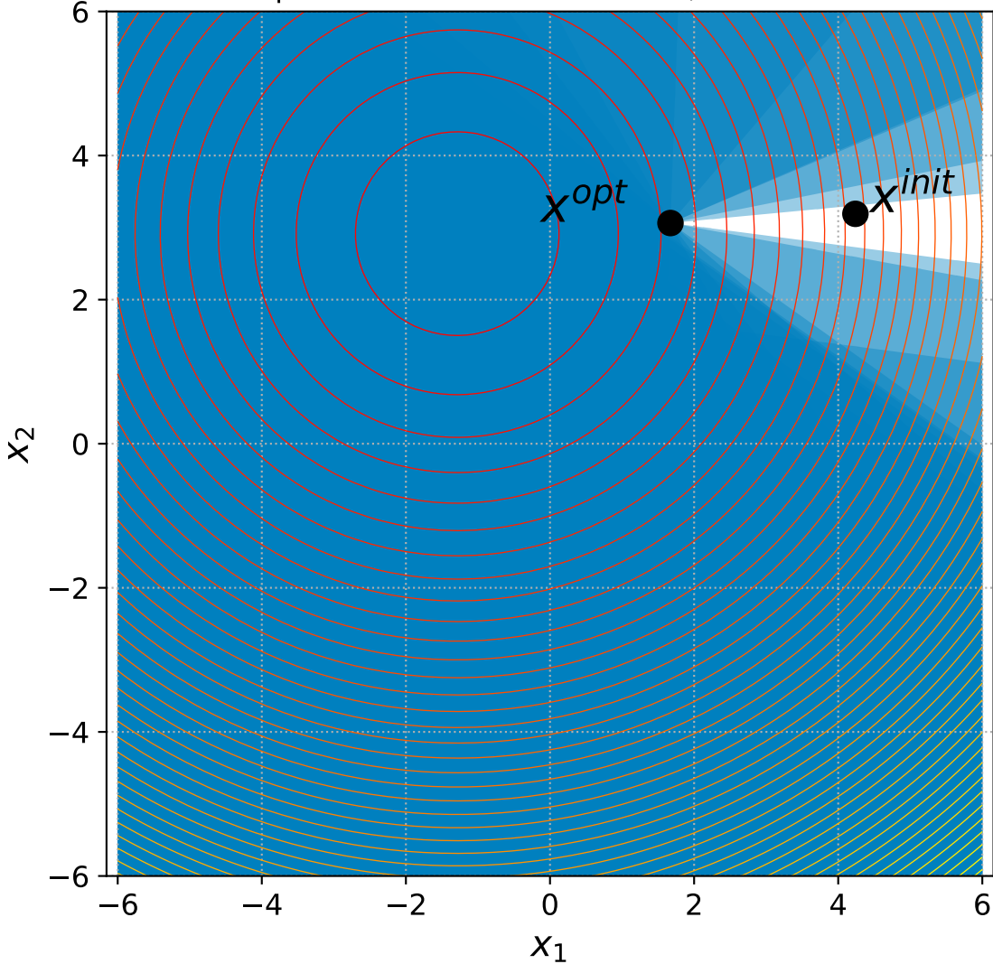
6 Sphere with 6+3n constraints, instance=9
