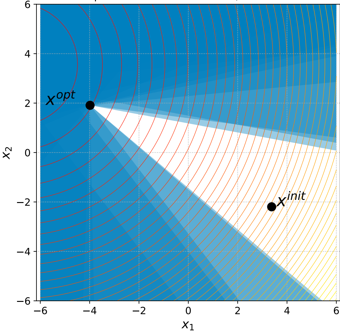
6 Sphere with 6+3n constraints, instance=4
