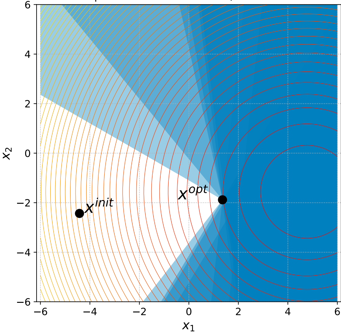
5 Sphere with 6+n constraints, instance=15
